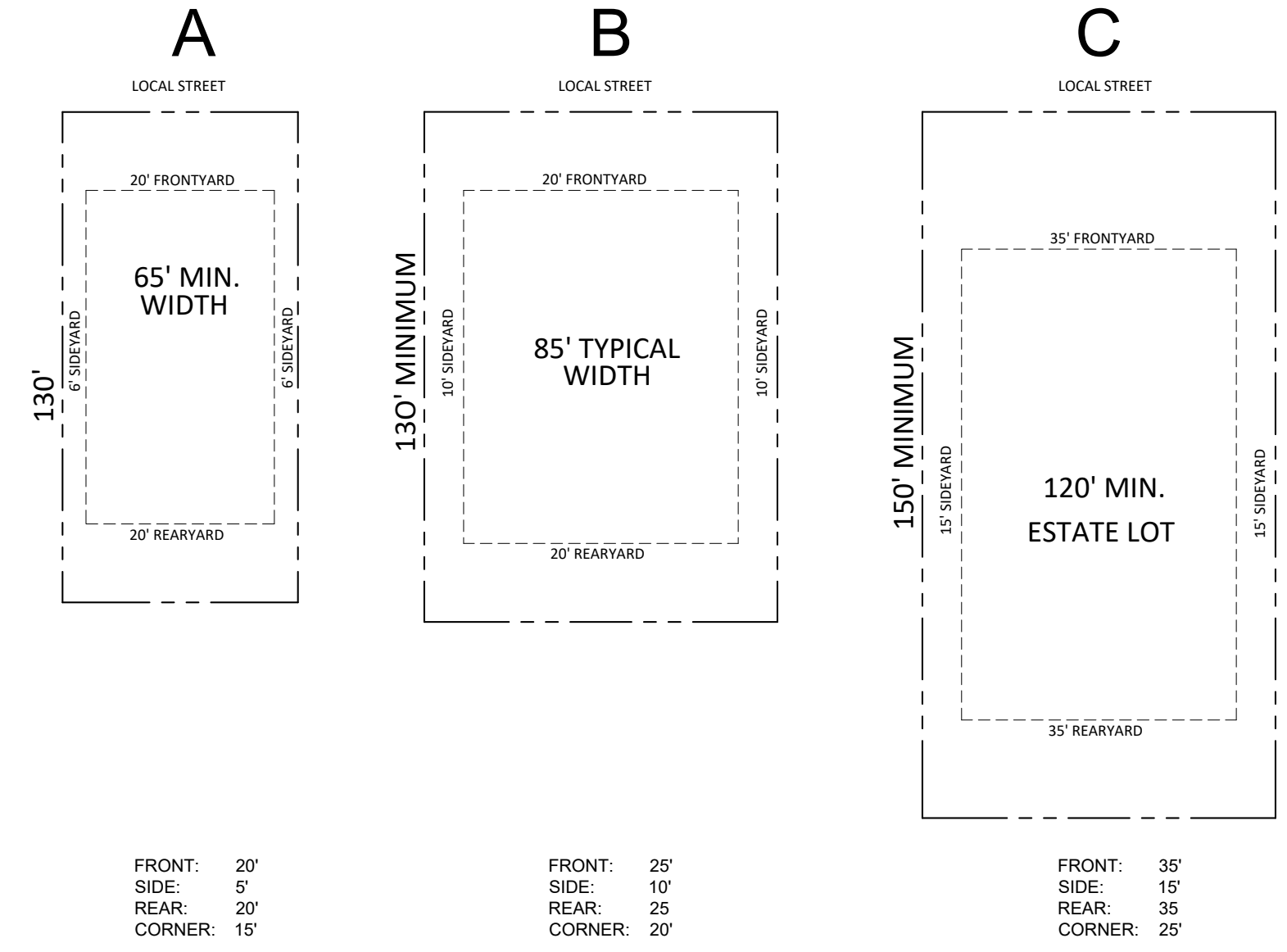
TYPICAL LOT DIAGRAMS AND SETBACKS
