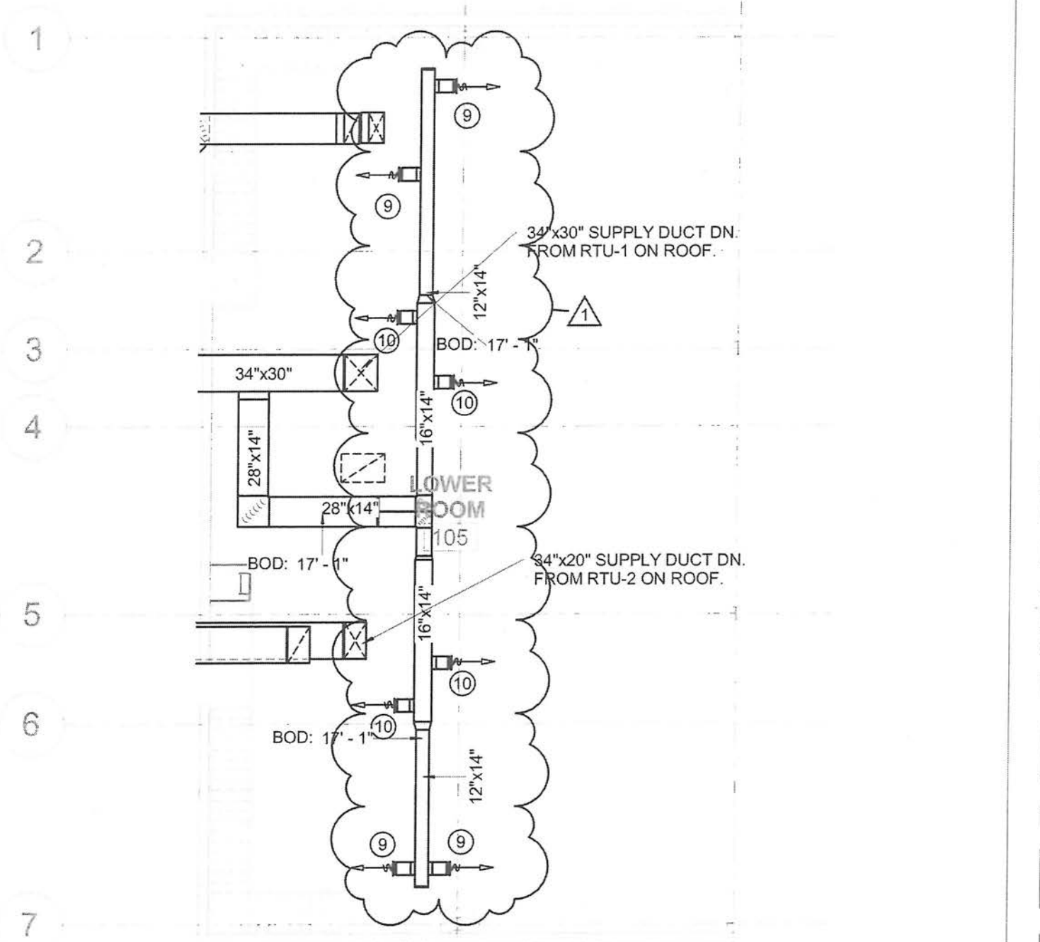
① UPPER LEVEL - MECHANICAL DUCTWORK PARTIAL PLAN 1" = 10'-0"
